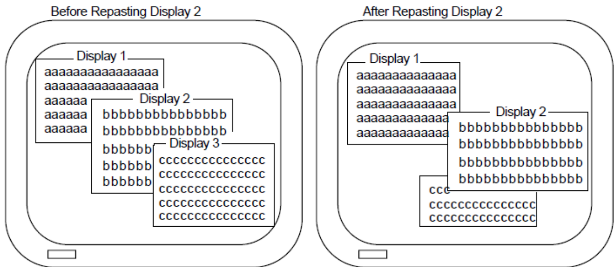
Figure 2.3. Repaste Operation
