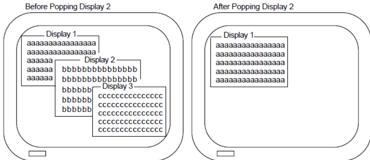
Figure 2.5. Pop Operation
