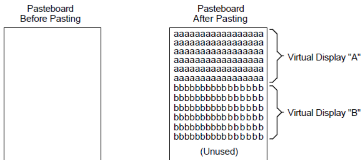
Figure 2.1. Paste Operation
