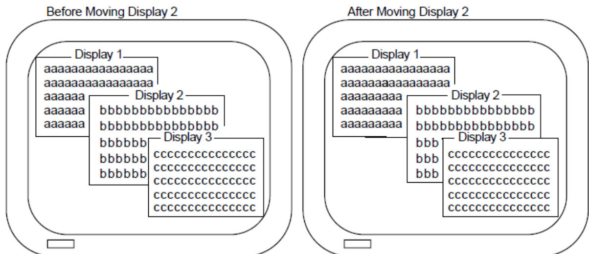
Figure 2.4. Move Operation
