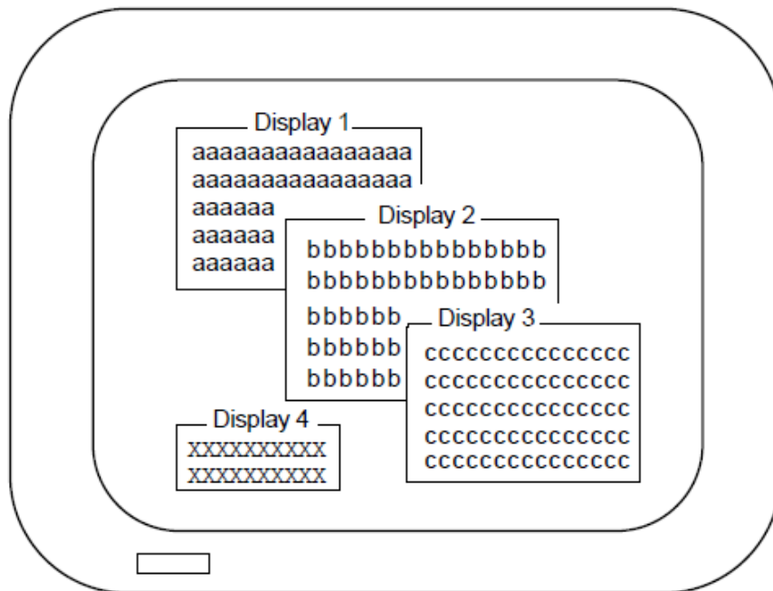
Figure 2.6. Occlusion Check
