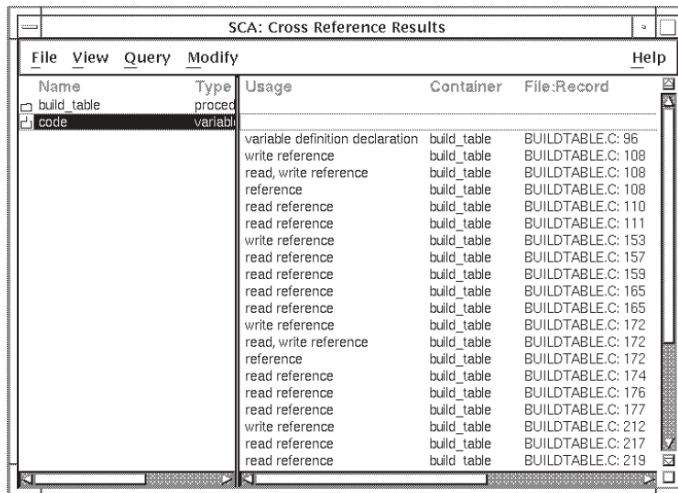
Figure 4.1. Cross-Referencing by Symbol Name
