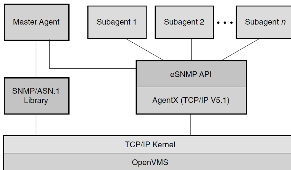
Figure 1.1. SNMP Architecture
