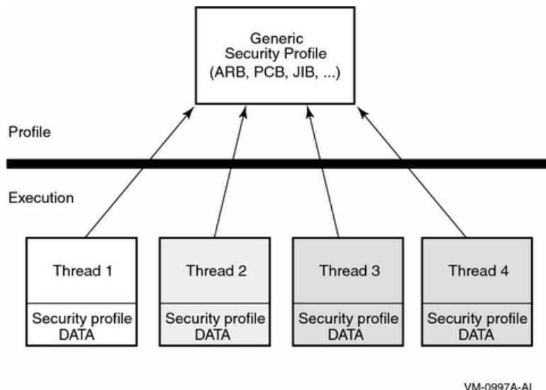
Figure 4.1. Previous Per-Thread Security Model
