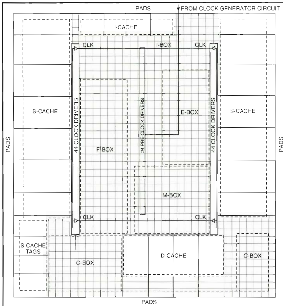
Figure 4 Metal 3 and Metal 4 Clock Grid
