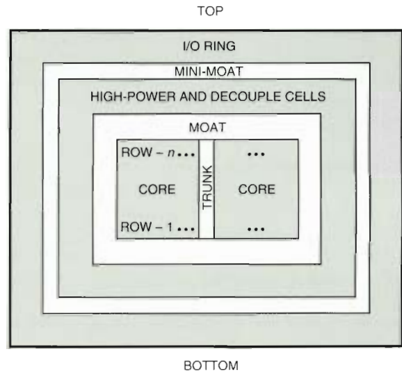
Figure 2 CSALT Die Architecture
